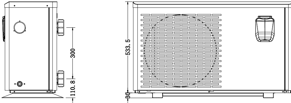
Heat pump 1401
